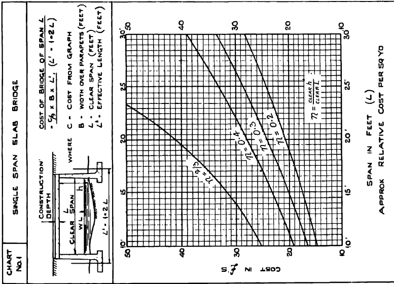
Fig. 253.—Cost of Single-span Slab Bridges.
